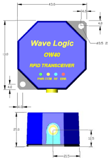
OW40 40mm OCTO WAVE™
